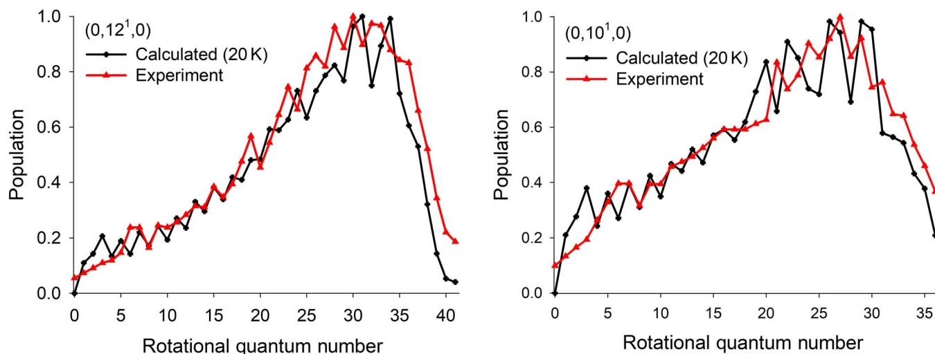
Fig. 3. Comparison of calculated and measured CO rotational distributions. The observed oscillatory and highly excited inverted product distributions are closely reproduced in the calculations. Simulated distributions for pure initial states (or lower beam temperatures) are even more oscillatory (see the Supplementary Materials).
